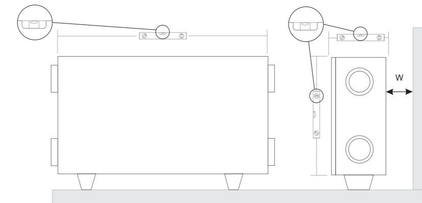
4.5.1 Montageposition: Horizontal Boden (W = 400 mm)
