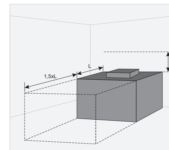
4.5.1 Montageposition: Horizontal Boden (W = 400 mm)
